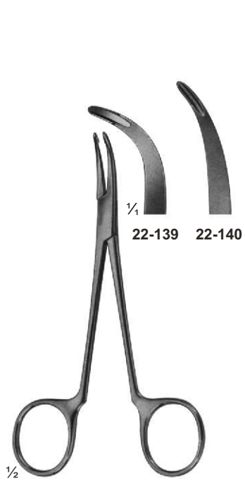
22-139 - 140 Synovcetomy rongeur width of jaws 2.0 mm 130 mm
